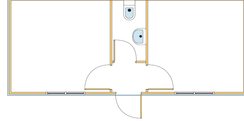
Dimension: 7.0x3.0 m Type: C707
