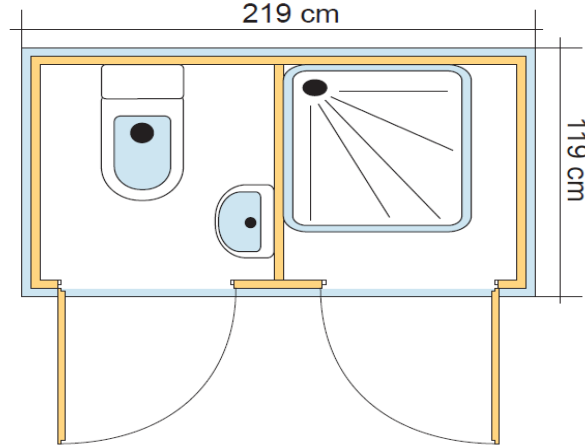
Dimension: 219x119 cm Type: W 104
