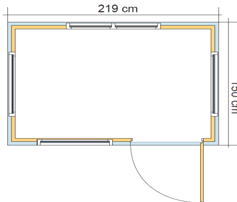
Dimension: 219x150 cm Type: S 102
