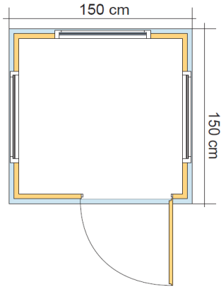
Dimension: 150x150 cm Type: S 101
