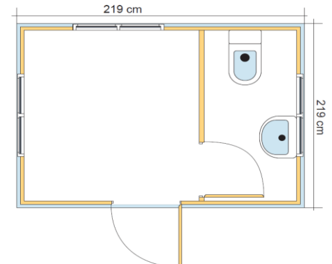
Dimension: 300x219 cm Type: S 104
