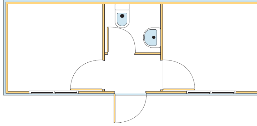
Dimension: 6.0x2.4 m Type: C606
